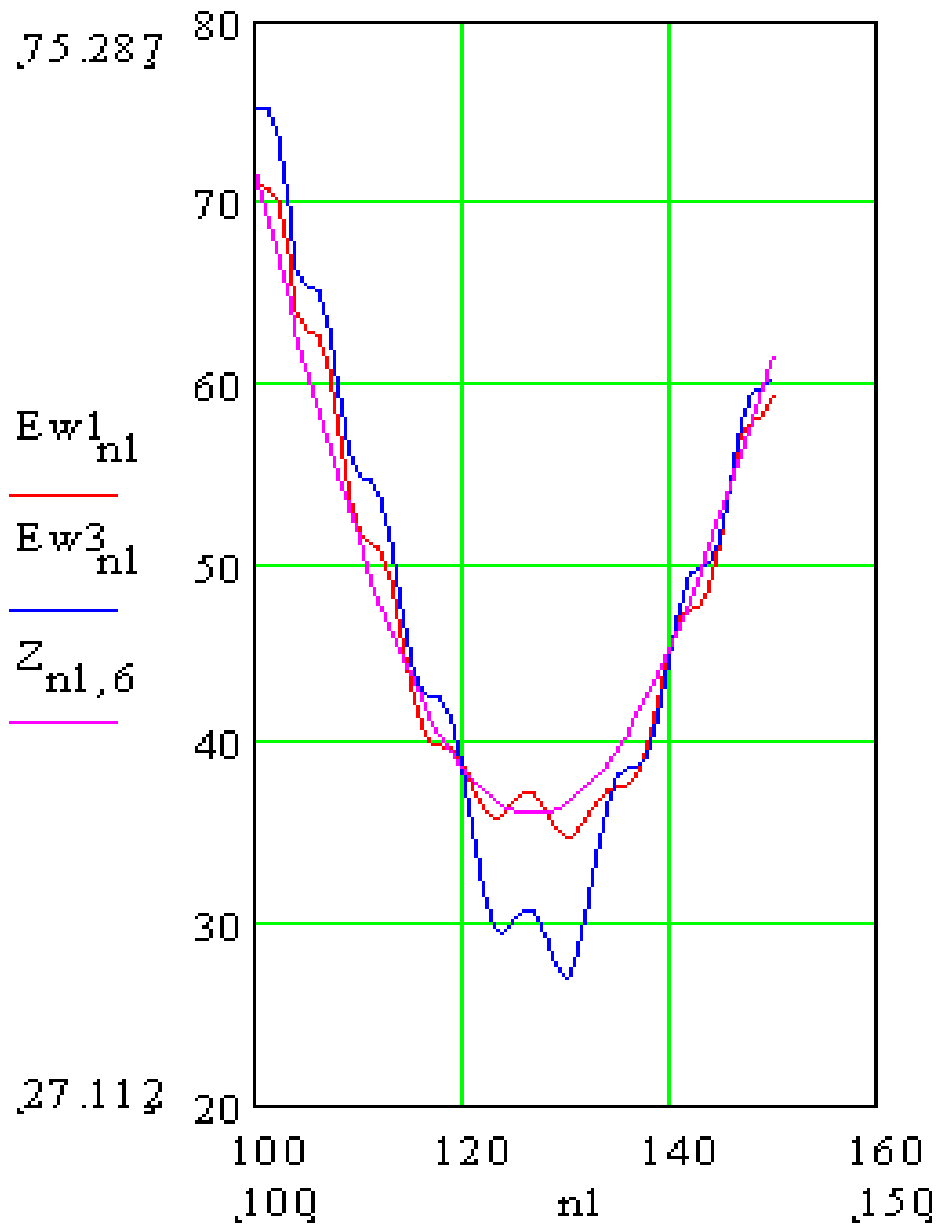
Fig. 12. Deterioration of accuracy of estimated Omega with higher order algorithms: 3 rd order estimate (Ew3 in blue) is worse than 1 st order estimate (Ew1 in red), actual in pink.
