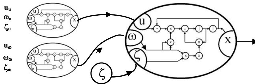
Fig. 3. Two of the input parameters of the final node are time varying modelled as 2 nd order hybrid integral recurrent nets.
