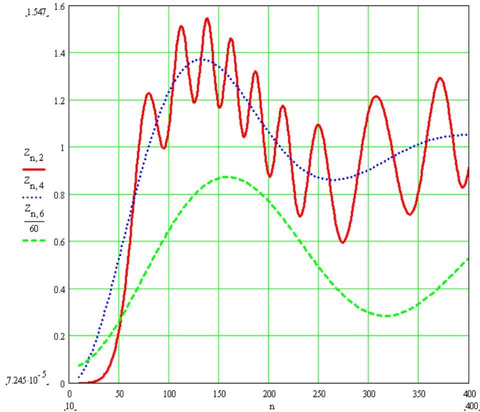
Fig. 5. Simulated trajectory of a hierarchical recurrent node (red trace), with 2 variable inputs: u (blue) and \omega (green)
