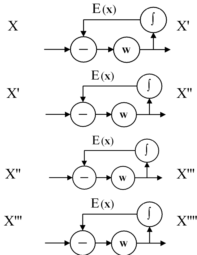
Fig. 6. A 4 th order recurrent network to abduct 1 st to 4 th time derivatives.
