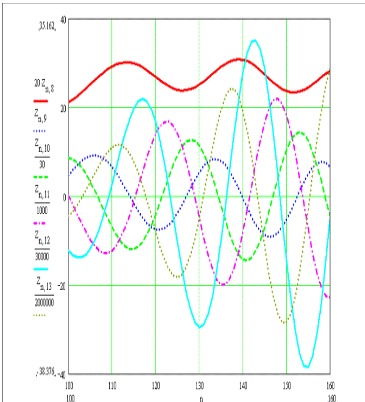
Fig. 8. A typical set of a recurrent node trajectory (red) and 5 higher order time derivatives x' to x'''' abducted from a simulation of an intelligent system trajectory
