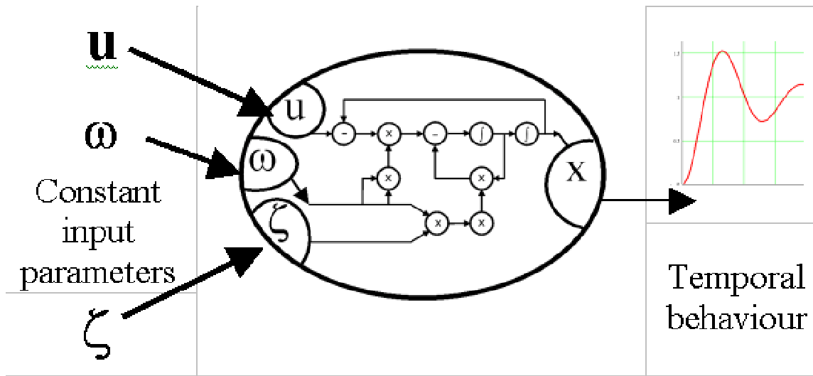
Fig. 2. Hybrid integral-recurrent net to model the temporal behaviour of the node in Fig. 1
