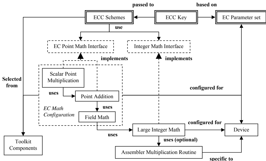
Figure 7: ECC System structure
