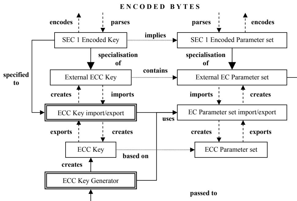
Figure 8: Generating, importing and exporting ECC keys and parameter sets
