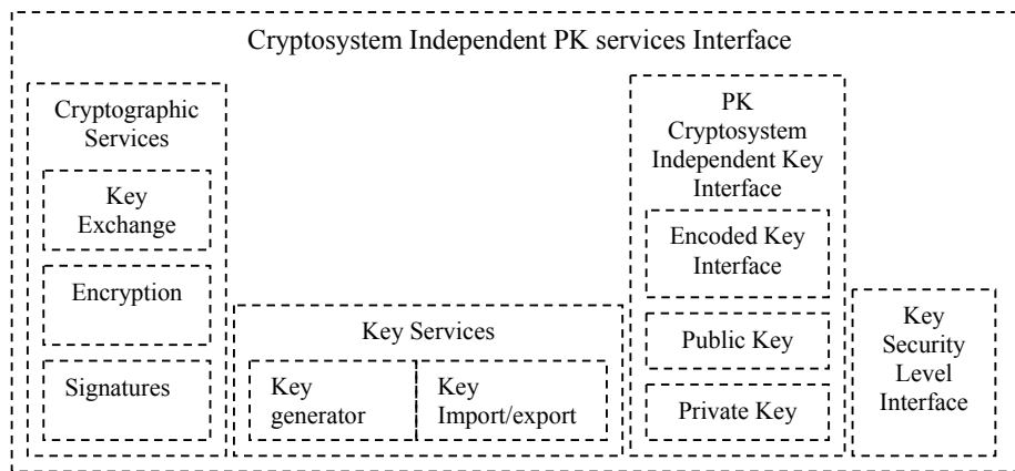
Figure 9: Generic Public Key Services interface
