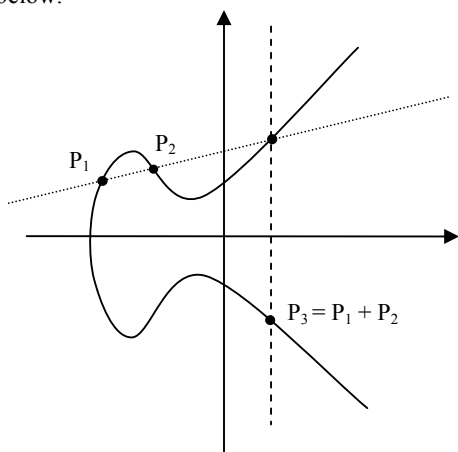
Figure 2: Illustration of adding two EC points.
