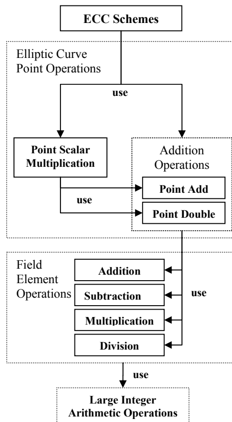
Figure 3: Hierarchy of required underlying mathematical operations
