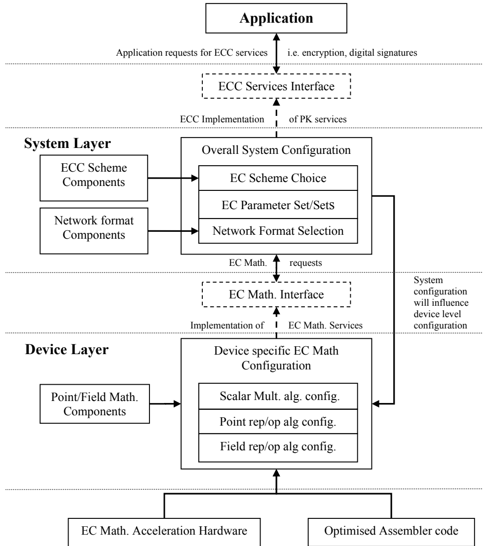
Figure 6: High level architecture of a two layered toolkit approach
