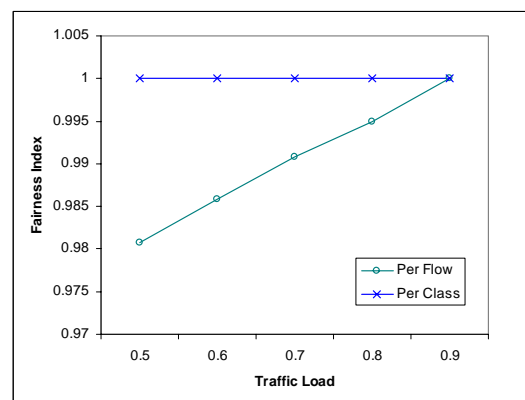
Figure 7: Fairness index
