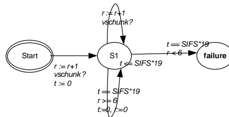
Figure 7: TA for Anchored Throughput
